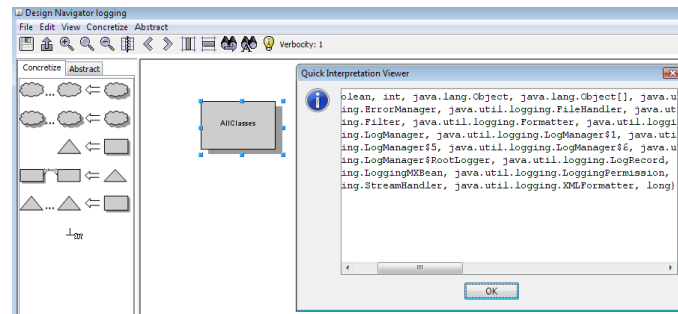
Screenshot 5 – AllClasses stands for all classes in package java.util.logging —Chart 1
