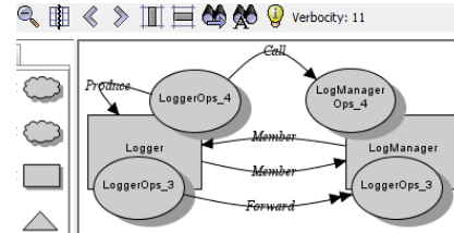
Chart 3 – Classes, methods, and correlations
